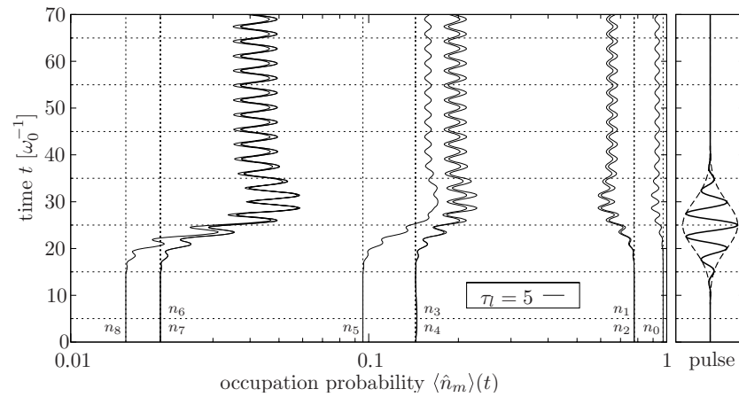
Figure 7. Mean-field dynamics of the HF orbital occupation probabilities \langle \hat{n}_m \rangle(t) = n_m for three charge carriers in a 2D artificial atom with the coupling parameter \lambda = 2.0 and inverse temperature \beta = 2 . The laser frequency is again near resonant, \omega_l = 1.25\omega_0 , and the pulse duration is \tau_l = 5 . In the initial state the occupation numbers n_1 and n_2 , n_3 and n_4 as well as n_6 and n_7 are practically pairwise degenerate, compare with the energy spectrum displayed in figure 6.
